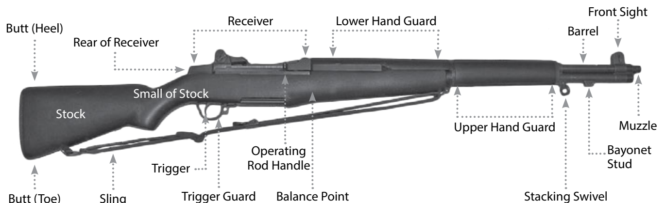
Figure 3-1a. M1 Garand Rifle Nomenclature
